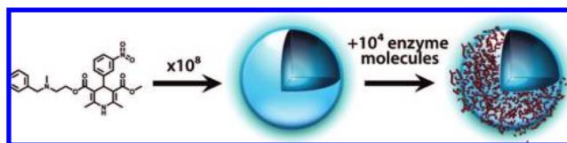
Figure 6. Model of aggregate structure and enzyme binding. Some organic molecules can form densely packed particles ( 10^8 small molecules per aggregate for larger particles) in aqueous media. Once formed, these larger particles sequester and then inhibit enzyme with a stoichiometry of approximately 10^4 enzyme molecules per aggregate. The surface of the aggregate is sufficient to accommodate all bound enzyme.
