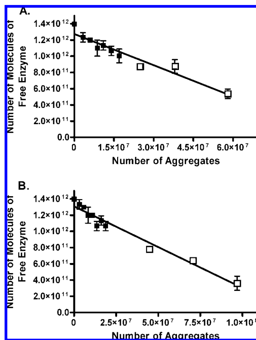
Figure 2. Correlation of \beta -lactamase inhibition to aggregate count for (A) nicardipine and (B) miconazole at 0.1% DMSO. The number of molecules of free enzyme is calculated as the product of percent activity and the total amount of enzyme in 1 mL. Aggregate count is measured by flow cytometry in a volume of 1.5 \mu\text{L} and extrapolated for 1 mL. Empty boxes represent aggregate counts that were extrapolated on the basis of a linear regression analysis of the measured aggregate count data points because the count was above the detection limit of the flow cytometer at higher concentrations of aggregating molecule. Free enzyme values are represented as the mean and standard deviation of three replicates. Aggregate counts are the mean of at least five measurements.
